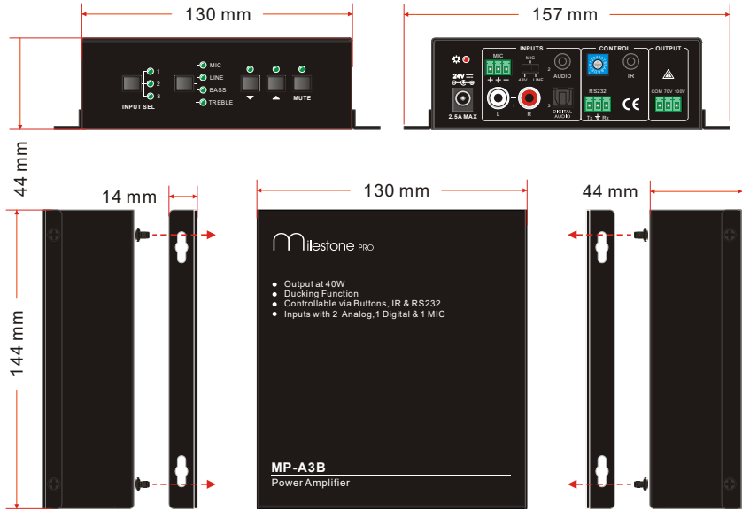
Figure 13 Panel Drawing
